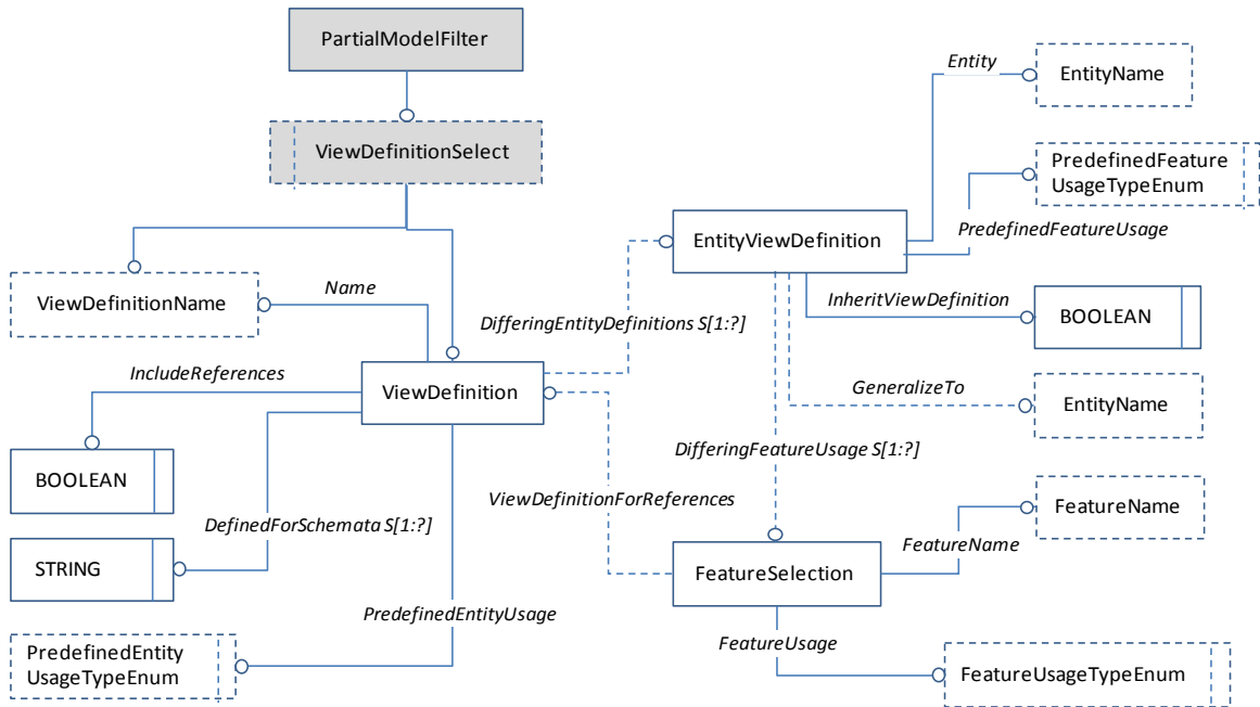
Fig. 4: Partial GMSD Diagram related to View Definitions (elements of minor importance are omitted)
